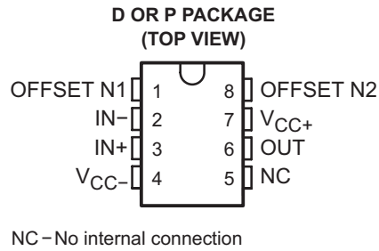
Pin Functions
